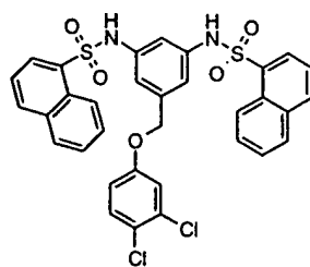
Compound # 7
